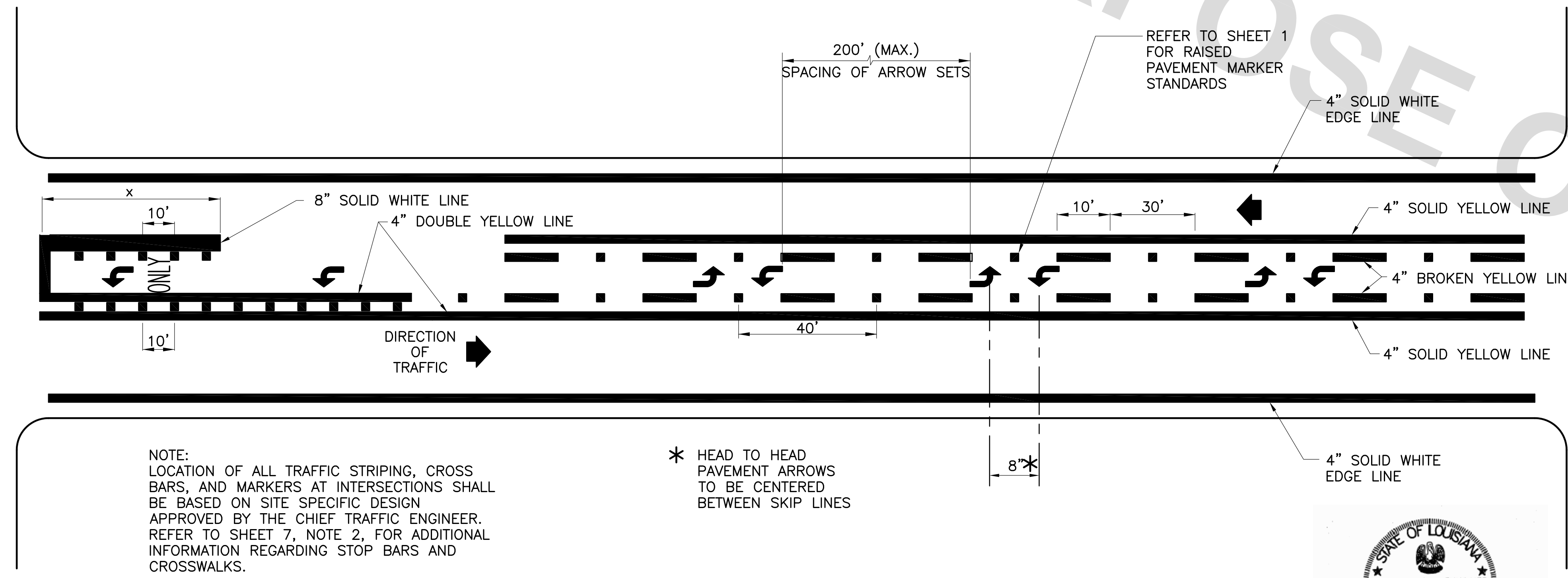
TWO WAY LEFT TURN LANE MARKINGS 3-LANE ROADWAY
