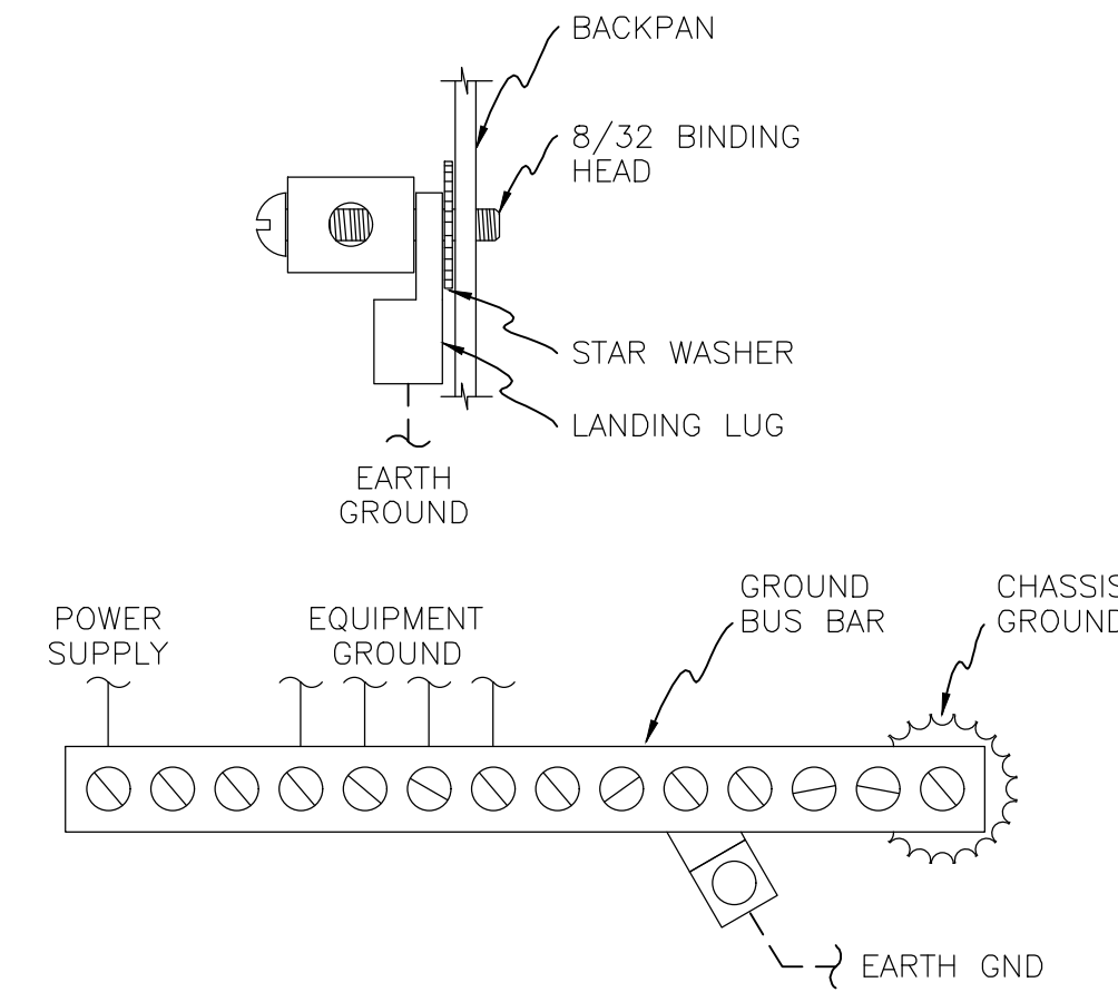
EQUIPMENT GROUNDING DETAIL (NOT TO SCALE)
